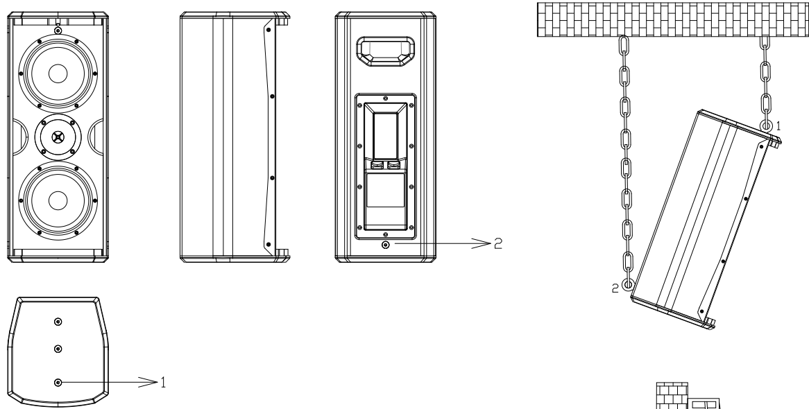
Fig. 9. S26 rigging points
