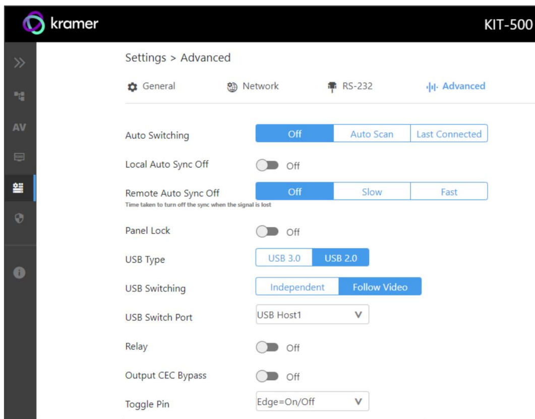
Figure 30: Settings Page – Advanced Tab
