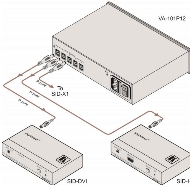
Figure 3: Connecting the VA-101P12, VA-102P12 Power Supply
