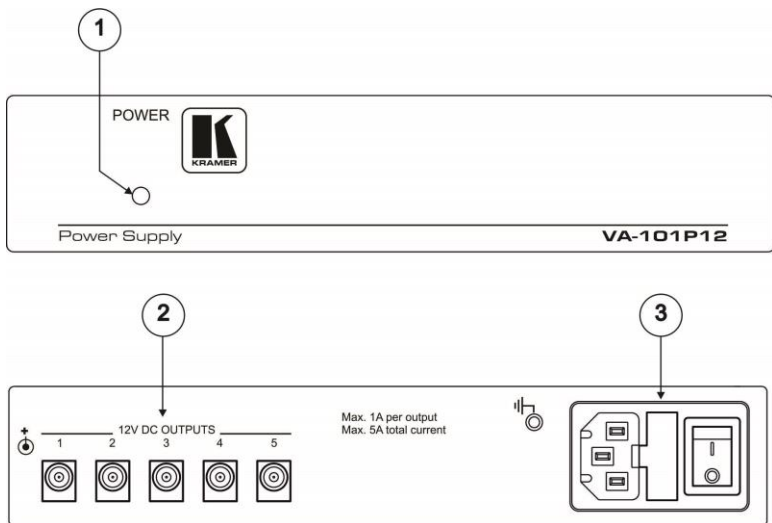
Figure 1: VA-101P12 5-Output 12V DC Power Supply
