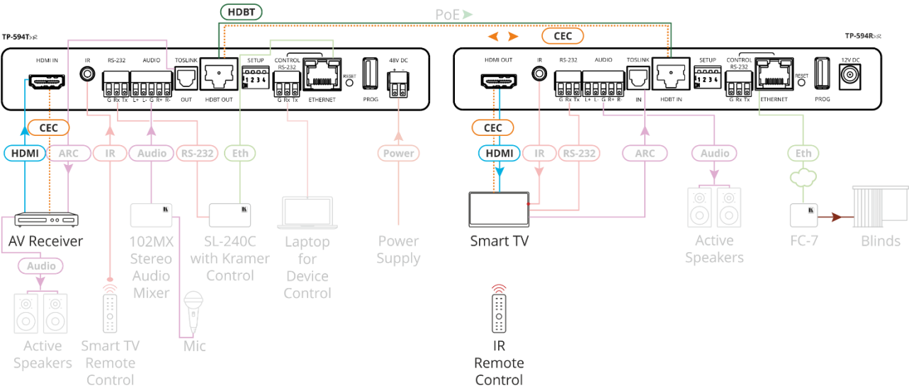
Figure 21: CEC End-to-End Extension
