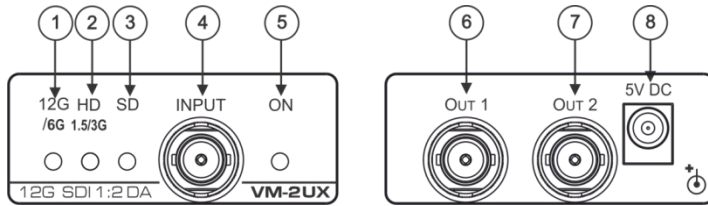
Figure 1: VM-2UX 12G SDI 1:2 DA
